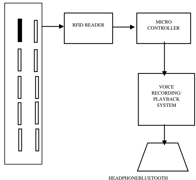
Fig 1.2 BLOCK DIAGRAM OF NAVIGATION UNIT
