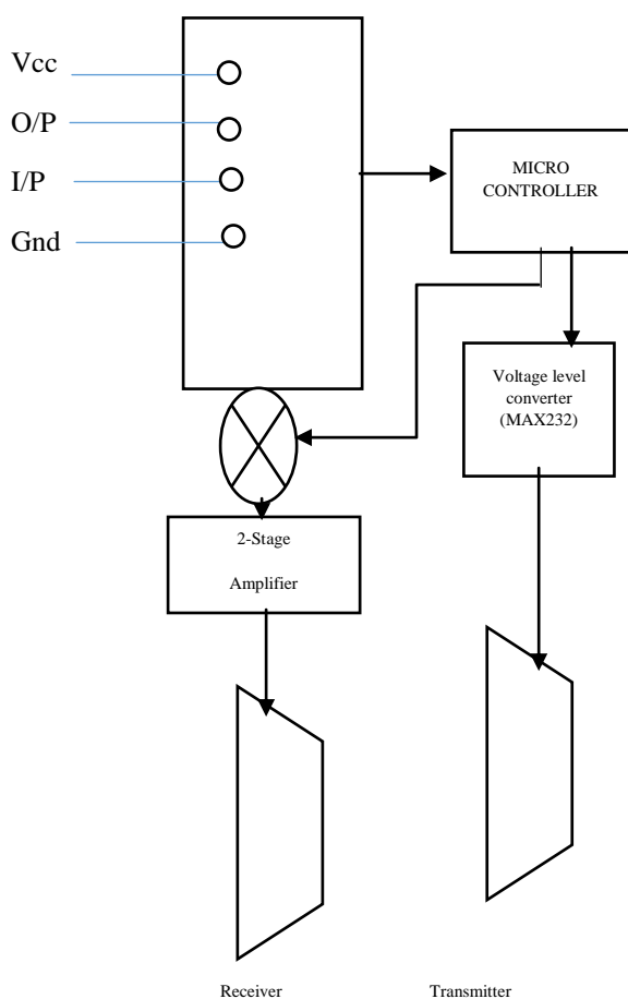
Fig 1.3 BLOCK DIAGRAM OF PROXIMITY SENSING UNIT
