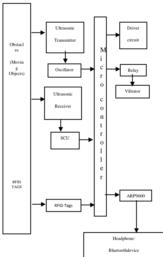
Fig 1.1 BLOCK DIAGRAM OF THE PROTOTYPE
