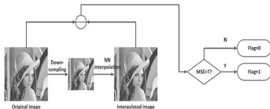
Fig. 5 An illustration of how to determine the type of an image
