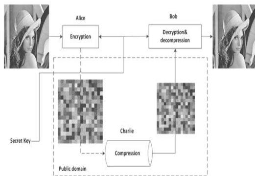
Fig. 2 Framework of combination of encryption and then compression
