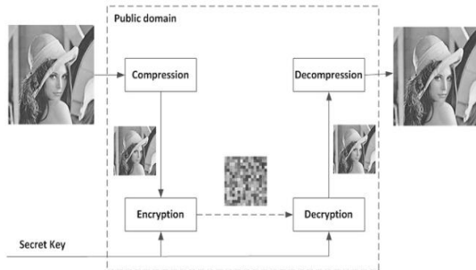
Fig. 1 Framework of general combination of compression and encryption
