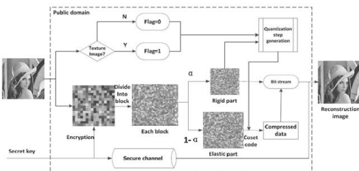
Fig. 4 Framework of proposed block-based compression in encryption domain
