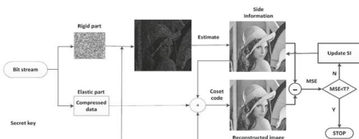
Fig. 6 Framework of proposed decompression and recovery method
