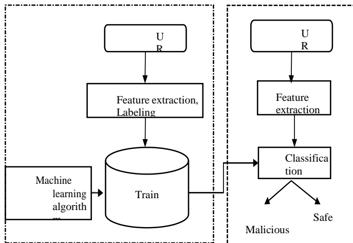
Figure 1. Malicious URL Detection Model using Machine Learning.
