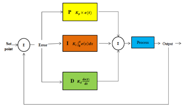
Fig. 1: Structure of PID Controller
