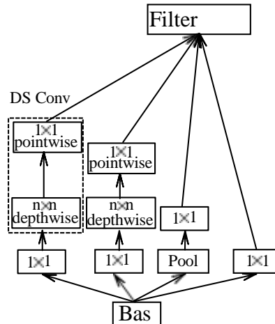
Figure 1. Basic architectures of implemented DL models.
