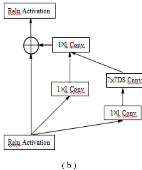
Figure 3. (a) Modified structures of InceptionResNet-A. (b) Structures of InceptionResNet-B of InceptionResNetV2 model.
